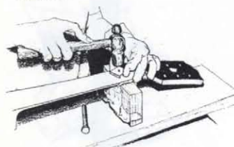
Positioning pin for fingerboard installation
