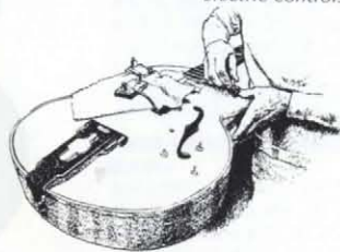
Installation of electric controls
